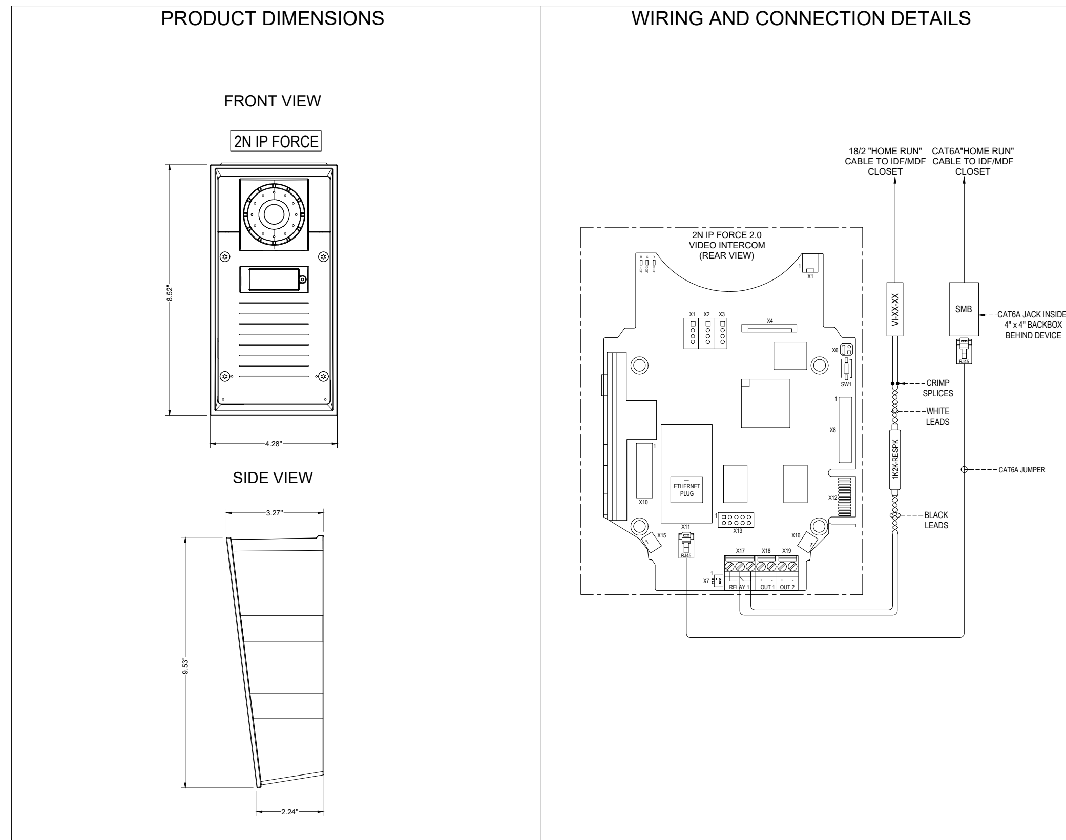
2 TYPICAL IP VIDEO INTERCOM (VI-XX-XX)
