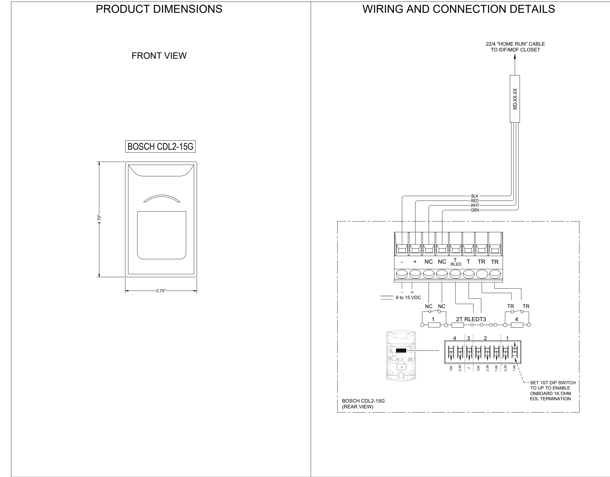
3 TYPICAL MOTION DETECTOR (MD-XX-XX)
