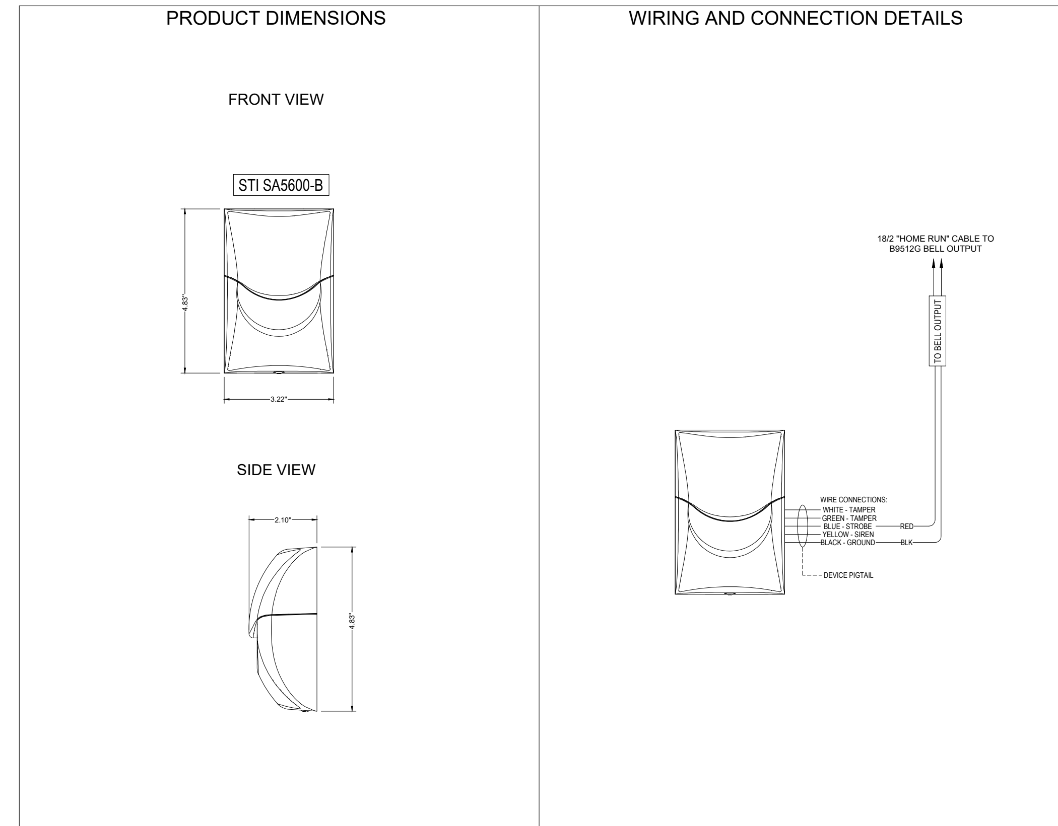
1 TYPICAL SIREN/STROBE DEVICE
